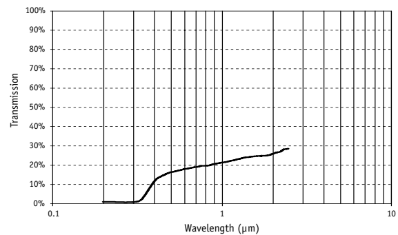
QEA Attenuator Spectral Transmission
