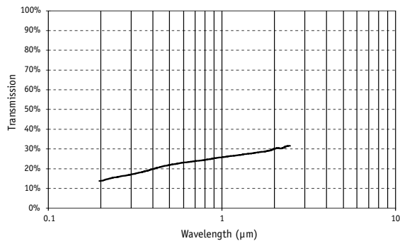
QEAS Attenuator Spectral Transmission
