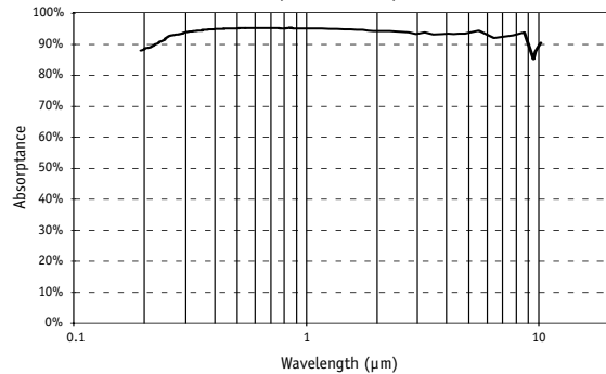
Broadband Black Absorber Spectral Absorption (QE/ED Series)
