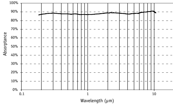
MB/UV High Energy Spectral Absorption (QE/ED Series)
