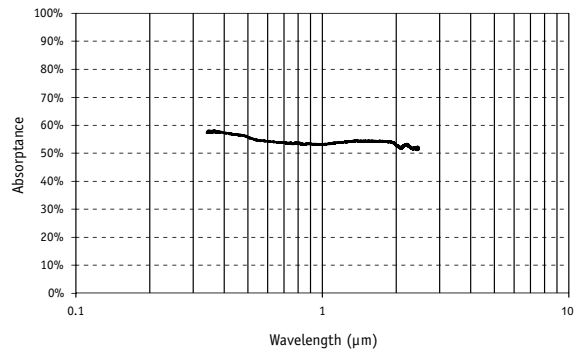
XLE4 Absorber Spectral Absorption
