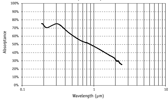
MT Coating Spectral Absorption (QE Series)
