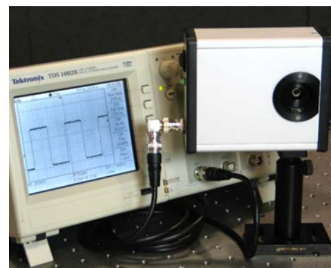
Fig. 2 QS-I-TEST and detector setup in the Radiometric mode for power measurement (W) of a chopped or modulated source.
