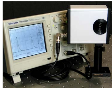
Fig. 1 QS-I-TEST and detector setup in Joulemeter mode for pulse energy measurement (J) of a pulsed source.
